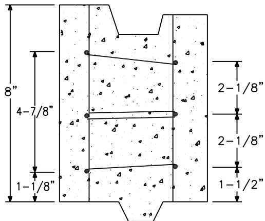
24" X 8" GRADE RING
