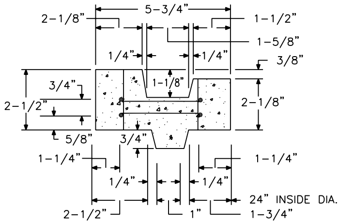
24" X 2 1/2" GRADE RING
