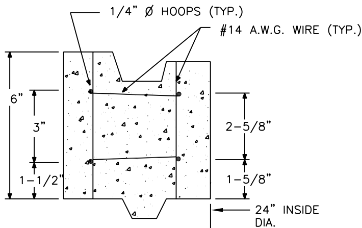
24" X 6" GRADE RING
