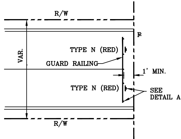
TYPICAL DEAD END
