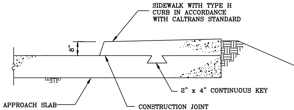
SECTION
