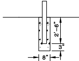
FOOTING DETAIL
