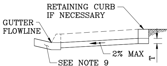
SECTION B-B SEE SHEET 1
