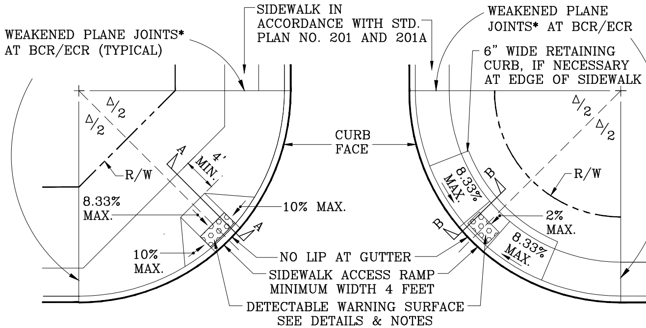
STRAIGHT CORNER CUT-OFF
