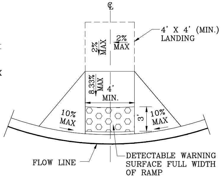
DETECTABLE WARNING SURFACE
